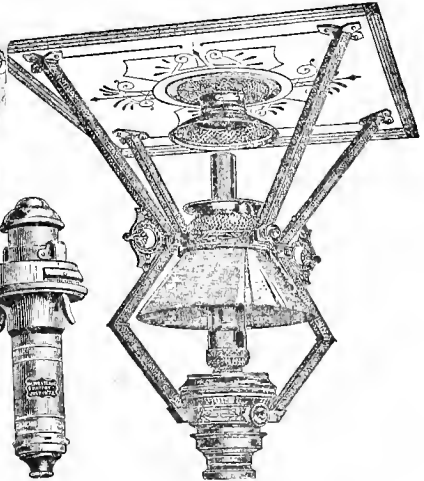
Fig. 3260. Drop over-all, 24 ins. Moehring's Center-draft Burner.
